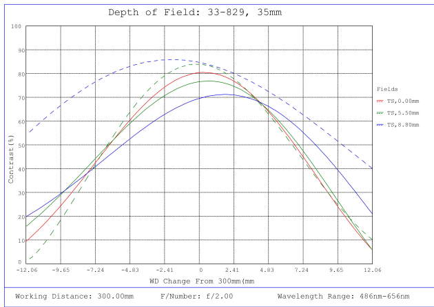
#33-829, 35mm f/2.0, HPI Series Fixed Focal Length Lens, Depth of Field Plot, 300mm Working Distance, f2
