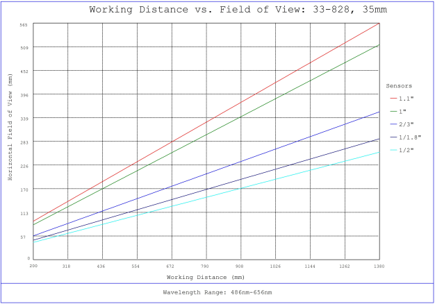
#33-828, 35mm f/1.8, HPi Series Fixed Focal Length Lens, Working Distance versus Field of View Plot
