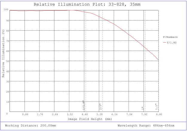
#33-828, 35mm f/1.8, HPi Series Fixed Focal Length Lens, Relative Illumination Plot
