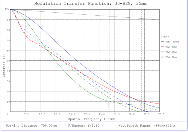
#33-828, 35mm f/1.8, HPi Series Fixed Focal Length Lens, Modulated Transfer Function (MTF) Plot, 750mm Working Distance, f1.8
