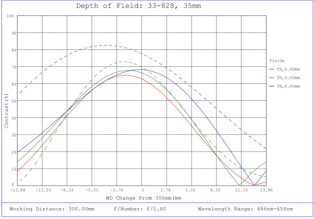
#33-828, 35mm f/1.8, HPi Series Fixed Focal Length Lens, Depth of Field Plot, 300mm Working Distance, f1.8
