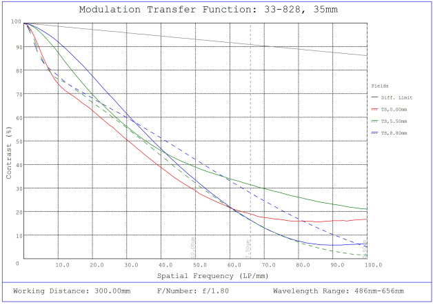
#33-828, 35mm f/1.8, HPi Series Fixed Focal Length Lens, Modulated Transfer Function (MTF) Plot, 300mm Working Distance, f1.8
