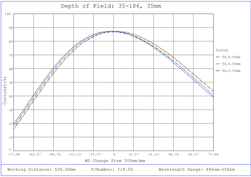
#35-186, 35mm, f/8.0 Cr Series Fixed Focal Length Lens, Depth of Field Plot, 500mm Working Distance, f8
