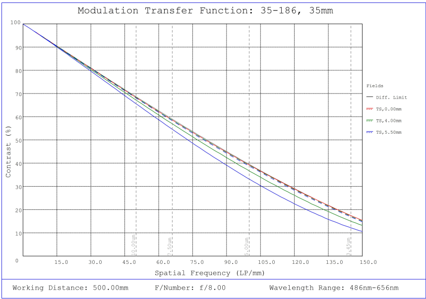
#35-186, 35mm, f/8.0 Cr Series Fixed Focal Length Lens, Modulated Transfer Function (MTF) Plot, 500mm Working Distance, f8
