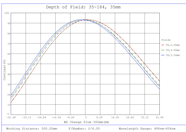
#35-184, 35mm, f/4.0 Cr Series Fixed Focal Length Lens, Depth of Field Plot, 500mm Working Distance, f4
