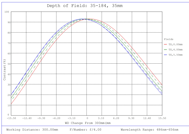
#35-184, 35mm, f/4.0 Cr Series Fixed Focal Length Lens, Depth of Field Plot, 300mm Working Distance, f4
