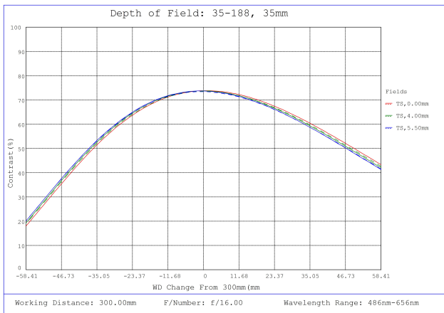
#35-188, 35mm, f/16 Cr Series Fixed Focal Length Lens, Depth of Field Plot, 300mm Working Distance, f16
