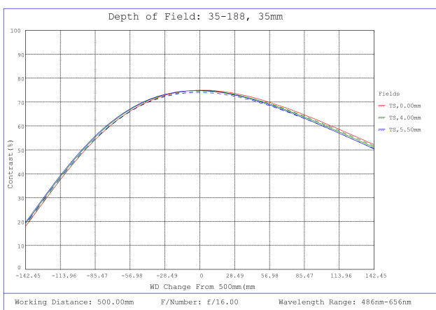
#35-188, 35mm, f/16 Cr Series Fixed Focal Length Lens, Depth of Field Plot, 500mm Working Distance, f16
