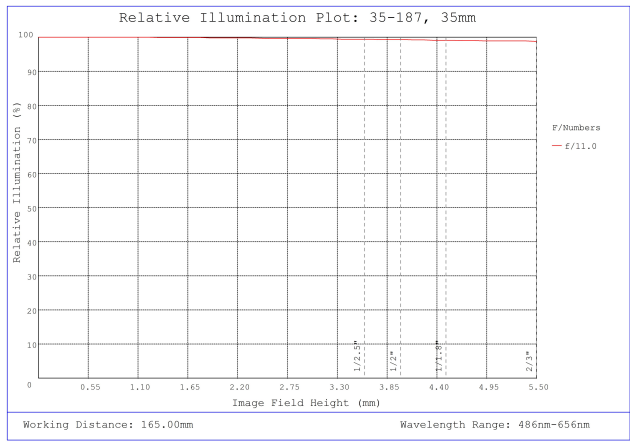
#35-187, 35mm, f/11 Cr Series Fixed Focal Length Lens, Relative Illumination Plot
