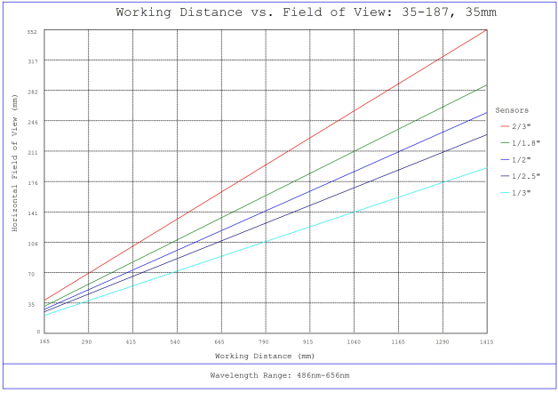
#35-187, 35mm, f/11 Cr Series Fixed Focal Length Lens, Working Distance versus Field of View Plot
