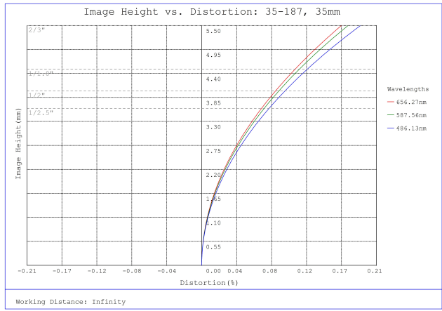
#35-187, 35mm, f/11 Cr Series Fixed Focal Length Lens, Distortion Plot
