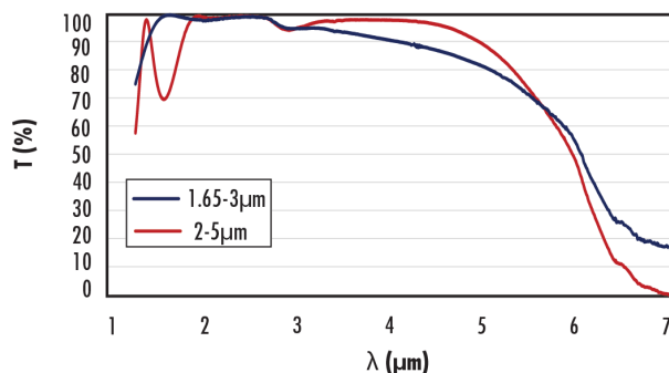
Infrared AR Coated Sapphire Windows 1mm Thickness
