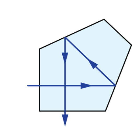
Penta Prism Ray Path
