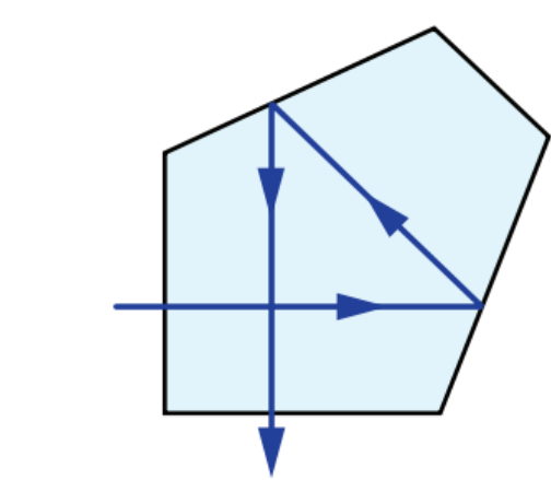
Penta Prism Ray Path
