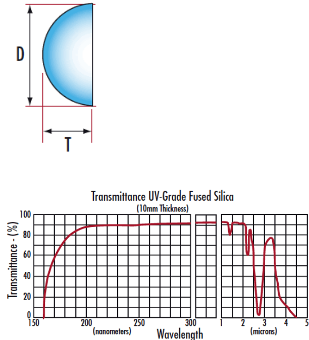
UV FS Transmission Curve
