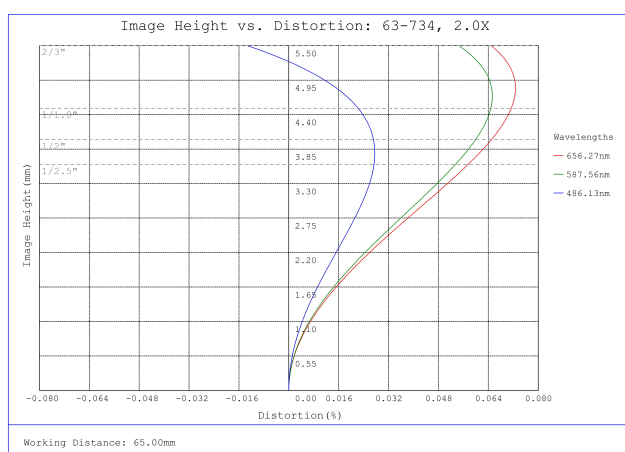
#63-734, 2X, 65mm WD CompactTL™ Telecentric Lens, Distortion Plot
