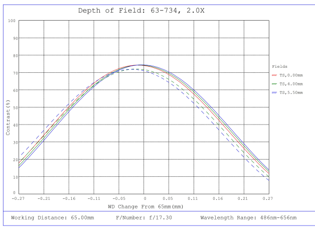
#63-734, 2X, 65mm WD CompactTL™ Telecentric Lens, Depth of Field Plot, 65mm Working Distance, f17.3
