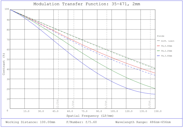
#35-471, 2mm FL f/5.6 IR-Cut Rugged Blue Series M12 Lens, Modulated Transfer Function (MTF) Plot, 100mm Working Distance, f5.6
