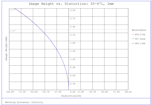
#35-471, 2mm FL f/5.6 IR-Cut Rugged Blue Series M12 Lens, Distortion Plot
