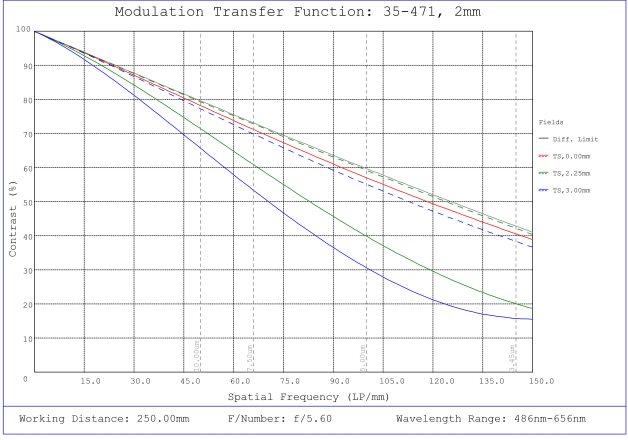
#35-471, 2mm FL f/5.6 IR-Cut Rugged Blue Series M12 Lens, Modulated Transfer Function (MTF) Plot, 250mm Working Distance, f5.6
