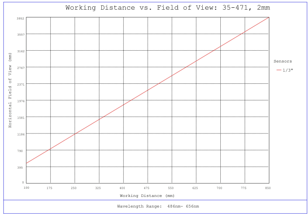
#35-471, 2mm FL f/5.6 IR-Cut Rugged Blue Series M12 Lens, Working Distance versus Field of View Plot
