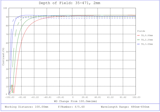
#35-471, 2mm FL f/5.6 IR-Cut Rugged Blue Series M12 Lens, Depth of Field Plot, 100mm Working Distance, f5.6
