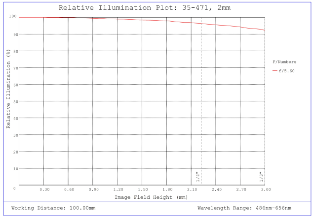
#35-471, 2mm FL f/5.6 IR-Cut Rugged Blue Series M12 Lens, Relative Illumination Plot
