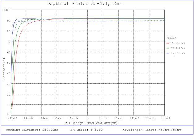
#35-471, 2mm FL f/5.6 IR-Cut Rugged Blue Series M12 Lens, Depth of Field Plot, 250mm Working Distance, f5.6
