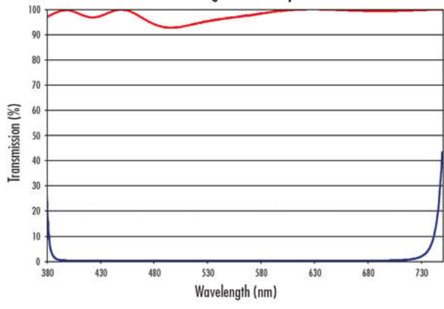
VIS Polarizing Cube Beamsplitters
