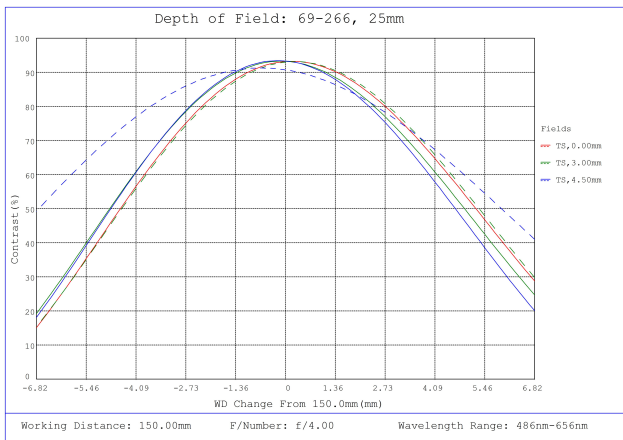
#69-266, 25mm FL f/4, Blue Series M12 Lens, Depth of Field Plot, 150mm Working Distance, f4
