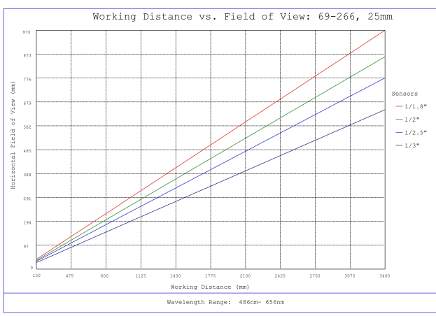
#69-266, 25mm FL f/4, Blue Series M12 Lens, Working Distance versus Field of View Plot
