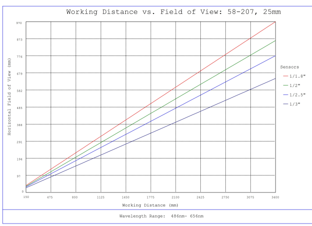
#58-207, 25mm FL f/2.5, Blue Series M12 Lens, Working Distance versus Field of View Plot
