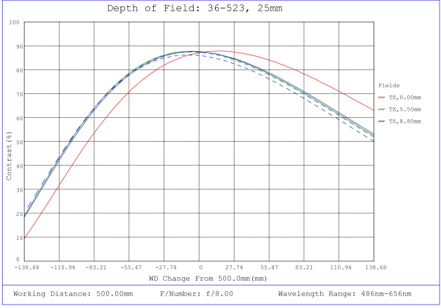
#36-523, 25mm f/8.0, HPr Series Fixed Focal Length Lens, Depth of Field Plot, 500mm Working Distance, f8
