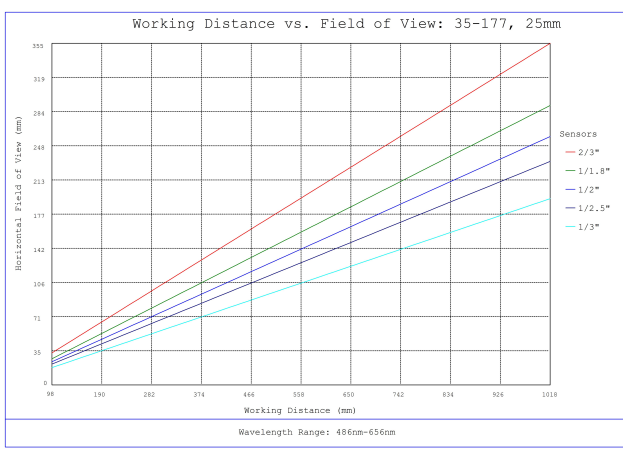
#35-177, 25mm, f/8 Cr Series Fixed Focal Length Lens, Working Distance versus Field of View Plot
