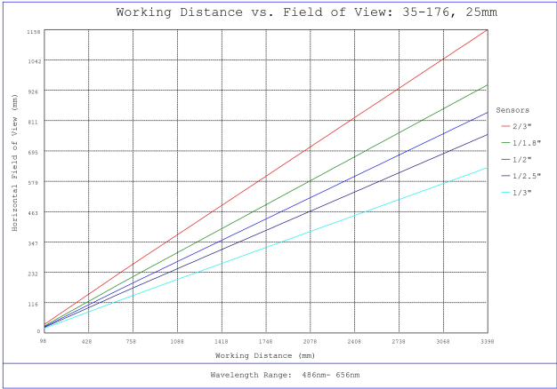
#35-176, 25mm, f/5.6 Cr Series Fixed Focal Length Lens, Working Distance versus Field of View Plot
