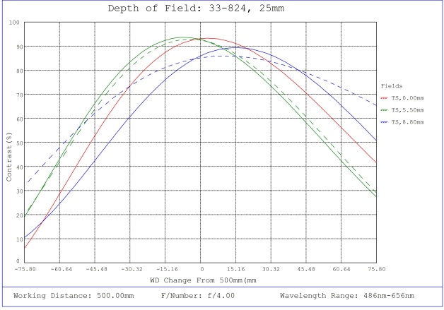
#33-824, 25mm f/4.0, HPi Series Fixed Focal Length Lens, Depth of Field Plot, 500mm Working Distance, f4
