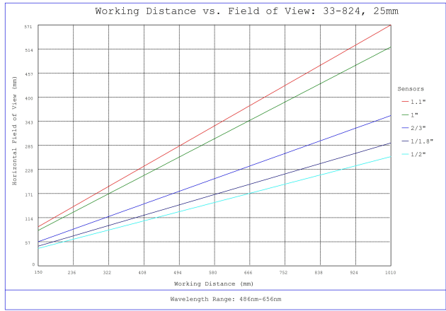
#33-824, 25mm f/4.0, HPI Series Fixed Focal Length Lens, Working Distance versus Field of View Plot
