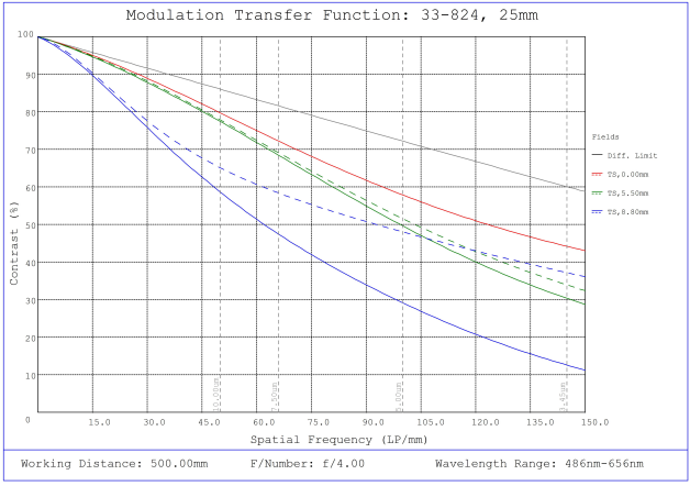
#33-824, 25mm f/4.0, HPi Series Fixed Focal Length Lens, Modulated Transfer Function (MTF) Plot, 500mm Working Distance, f4
