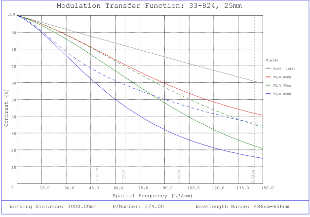
#33-824, 25mm f/4.0, HPi Series Fixed Focal Length Lens, Modulated Transfer Function (MTF) Plot, 1000mm Working Distance, f4
