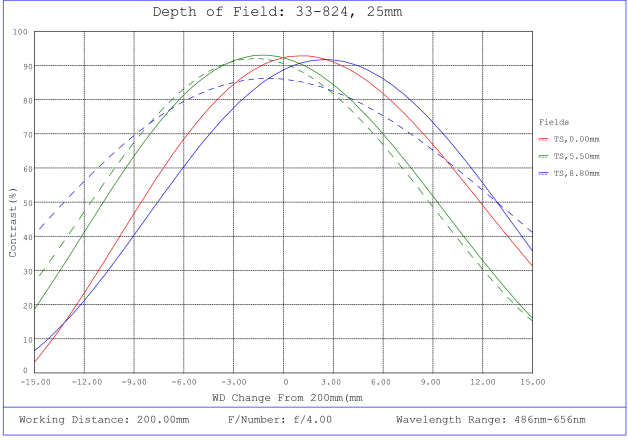
#33-824, 25mm f/4.0, HPi Series Fixed Focal Length Lens, Depth of Field Plot, 200mm Working Distance, f4
