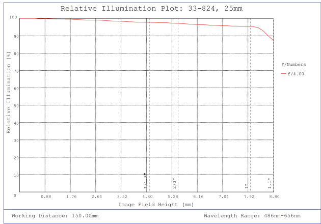
#33-824, 25mm f/4.0, HPI Series Fixed Focal Length Lens, Relative Illumination Plot
