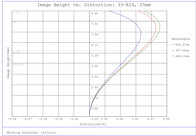
#33-824, 25mm f/4.0, HPI Series Fixed Focal Length Lens, Distortion Plot
