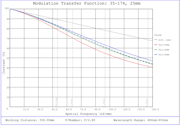
#35-174, 25mm, f/2.8 Cr Series Fixed Focal Length Lens, Modulated Transfer Function (MTF) Plot, 350mm Working Distance, f2.8
