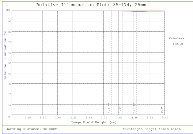
#35-174, 25mm, f/2.8 Cr Series Fixed Focal Length Lens, Relative Illumination Plot
