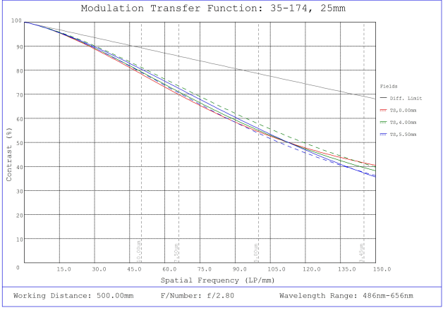
#35-174, 25mm, f/2.8 Cr Series Fixed Focal Length Lens, Modulated Transfer Function (MTF) Plot, 500mm Working Distance, f2.8
