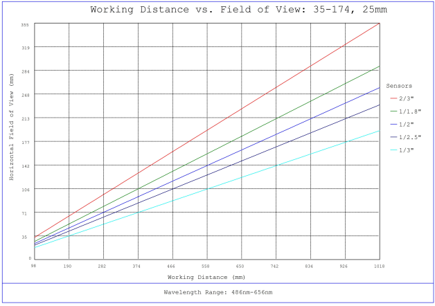
#35-174, 25mm, f/2.8 Cr Series Fixed Focal Length Lens, Working Distance versus Field of View Plot
