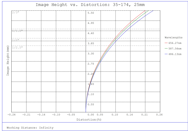
#35-174, 25mm, f/2.8 Cr Series Fixed Focal Length Lens, Distortion Plot
