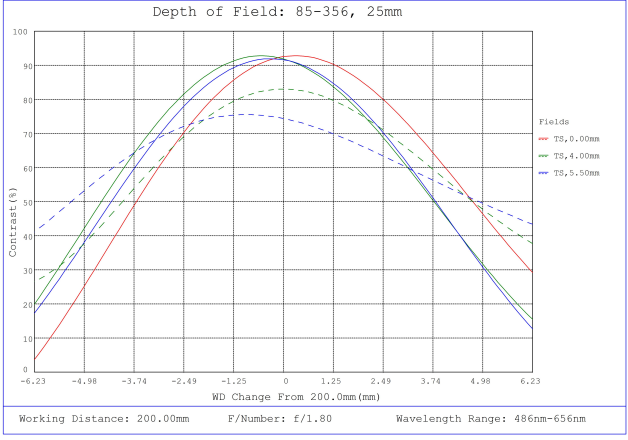
#85-356, 25mm, f/1.8 Ci Series Fixed Focal Length Lens, Depth of Field Plot, 200mm Working Distance, f1.8
