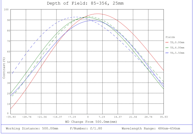
#85-356, 25mm, f/1.8 Ci Series Fixed Focal Length Lens, Depth of Field Plot, 500mm Working Distance, f1.8
