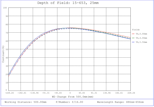
#15-653, 25mm, f/16 Cw Series Fixed Focal Length Lens, Depth of Field Plot, 500mm Working Distance, f16
