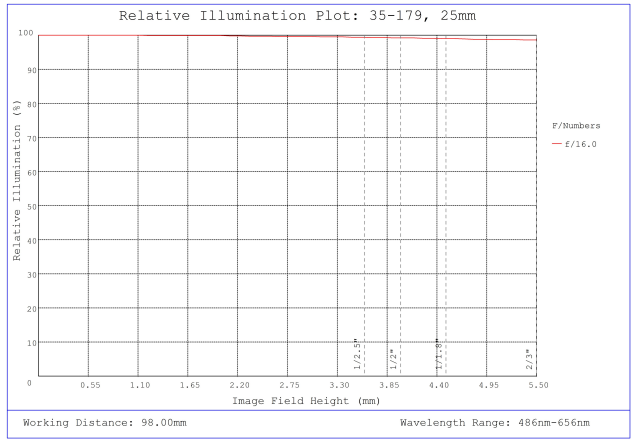
#35-179, 25mm, f/16 Cr Series Fixed Focal Length Lens, Relative Illumination Plot
