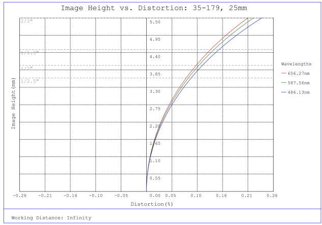
#35-179, 25mm, f/16 Cr Series Fixed Focal Length Lens, Distortion Plot
