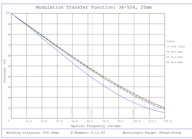
#36-524, 25mm f/11.0, HPr Series Fixed Focal Length Lens, Modulated Transfer Function (MTF) Plot, 500mm Working Distance, f11
