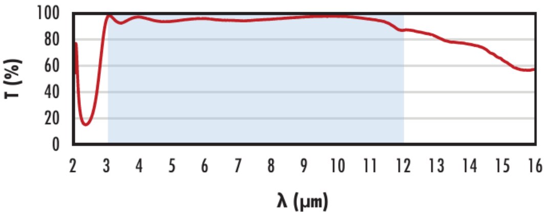
Ge with 3-12μm AR Coating Typical Transmission
