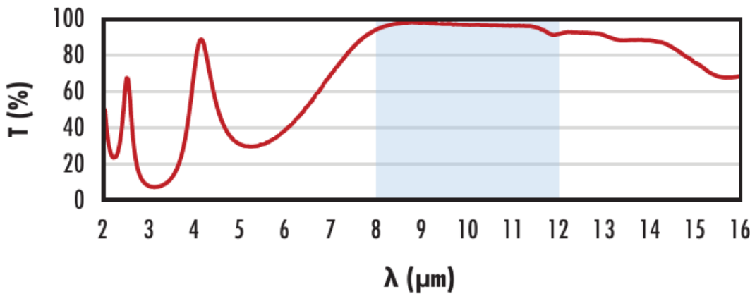
8-12μm AR Coated Germanium Typical Transmission
