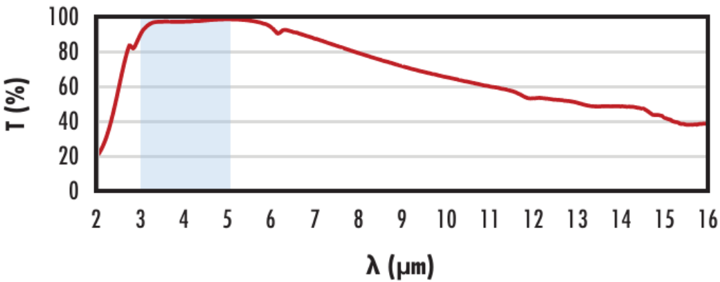
Ge with 3-5μm AR Coating Typical Transmission
