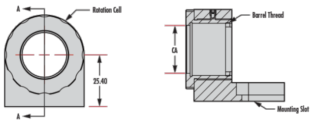
L-Slot Type (#36-411 & #36-417) Optic Rotation
