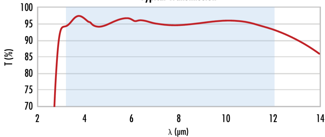
ZnSe with 3-12 \mu\text{m} AR Coating Typical Transmission
