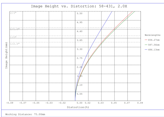
#58-431, 2.0X SilverTL™ Telecentric Lens, Distortion Plot
