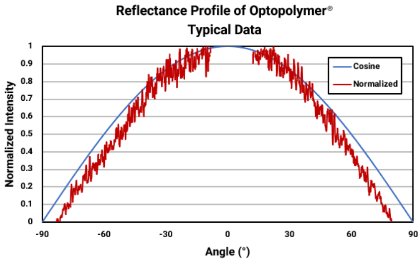
Typical, normalized reflectance profile of Optopoltmr®, showing near Lambertian properties. The gap in data is due to the detector crossing the path of the incident beam.
