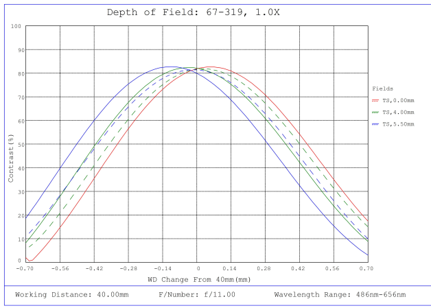
#67-319, 1X, 40mm WD, In-Line CompactTL™ Telecentric Lens, Depth of Field Plot, 40mm Working Distance, f11
