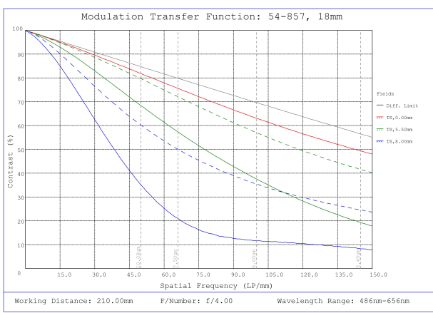
#54-857, 18mm DG Series Fixed Focal Length Lens, Modulated Transfer Function (MTF) Plot, 210mm Working Distance, f4
