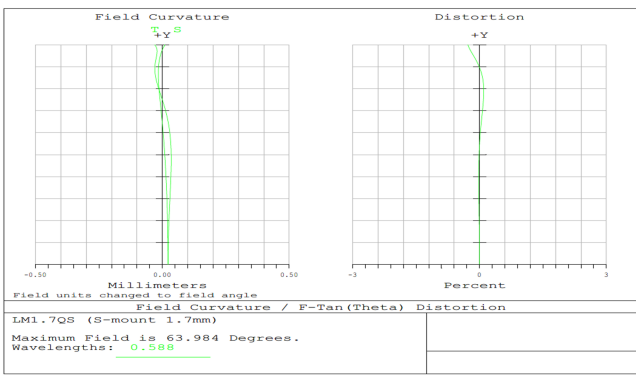
1.7mm FL, f/2.5, Low Distortion M12 Lens, Distortion Plot
