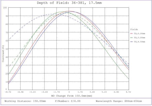
#36-381, 17.5mm FL f/4, Rugged Blue Series M12 Lens, Depth of Field Plot, 150mm Working Distance, f4
