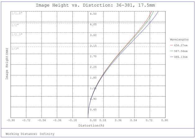
#36-381, 17.5mm FL f/4, Rugged Blue Series M12 Lens, Distortion Plot
