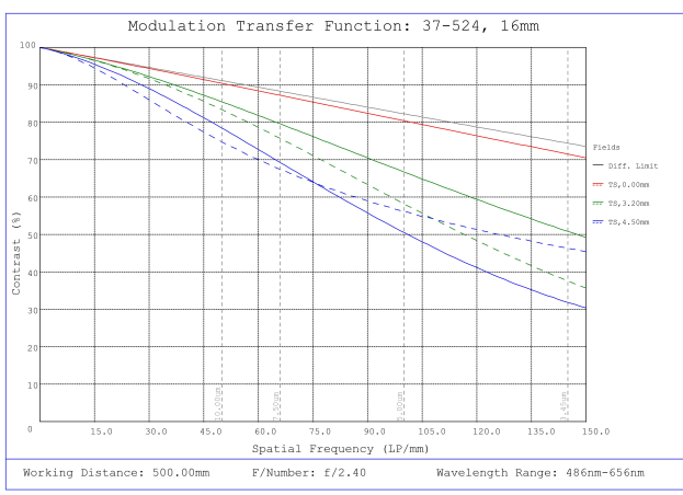
#37-524, 16mm FL, Liquid Lens M12 Lens, Modulated Transfer Function (MTF) Plot, 500mm Working Distance, f2.4
