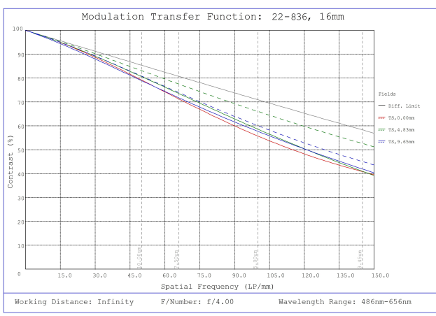
#22-836 - 16mm Focal Length, UAV Series Fixed Focal Length Lens, Modulated Transfer Function (MTF) Plot, Infinity Working Distance, f4
