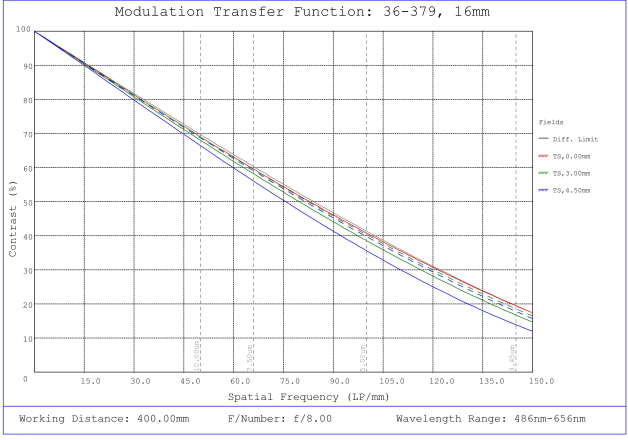
#36-379, 16mm FL f/8.0 Rugged Blue Series M12 Lens, Modulated Transfer Function (MTF) Plot, 400mm Working Distance, f8
