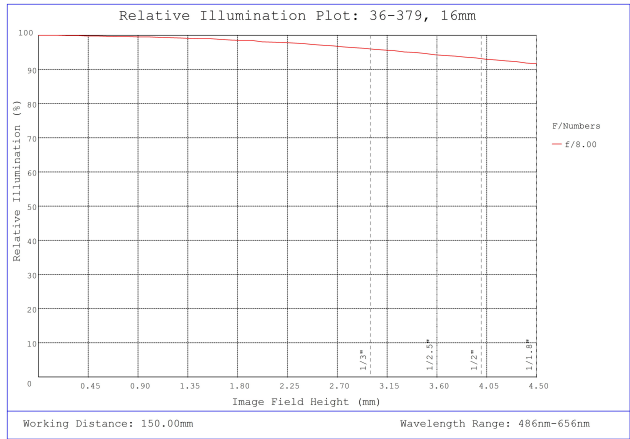
#36-379, 16mm FL f/8.0 Rugged Blue Series M12 Lens, Relative Illumination Plot
