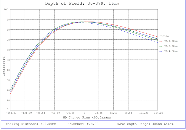
#36-379, 16mm FL f/8.0 Rugged Blue Series M12 Lens, Depth of Field Plot, 400mm Working Distance, f8
