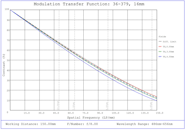
#36-379, 16mm FL f/8.0 Rugged Blue Series M12 Lens, Modulated Transfer Function (MTF) Plot, 150mm Working Distance, f8
