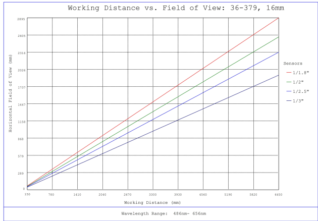
#36-379, 16mm FL f/8.0 Rugged Blue Series M12 Lens, Working Distance versus Field of View Plot
