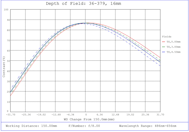
#36-379, 16mm FL f/8.0 Rugged Blue Series M12 Lens, Depth of Field Plot, 150mm Working Distance, f8
