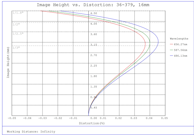
#36-379, 16mm FL f/8.0 Rugged Blue Series M12 Lens, Distortion Plot
