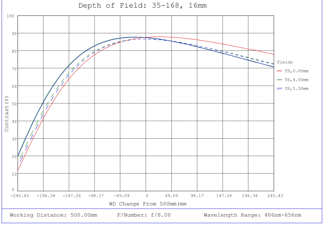
#35-168, 16mm, f/8 Cr Series Fixed Focal Length Lens, Depth of Field Plot, 500mm Working Distance, f8
