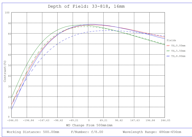
#33-818, 16mm f/8, HPI Series Fixed Focal Length Lens, Depth of Field Plot, 500mm Working Distance, f8
