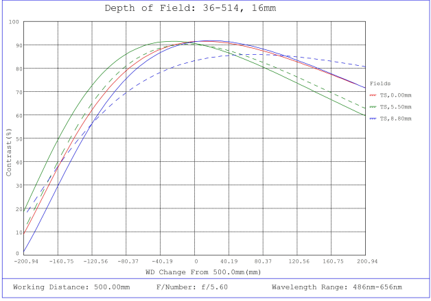
#36-514, 16mm f/5.6, HPr Series Fixed Focal Length Lens, Depth of Field Plot, 500mm Working Distance, f5.6
