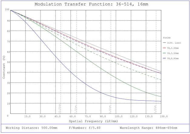
#36-514, 16mm f/5.6, HPr Series Fixed Focal Length Lens, Modulated Transfer Function (MTF) Plot, 500mm Working Distance, f5.6
