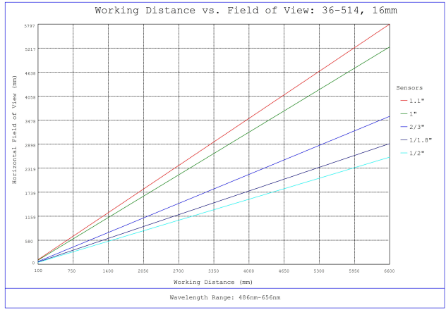
#36-514, 16mm f/5.6, HPr Series Fixed Focal Length Lens, Working Distance versus Field of View Plot
