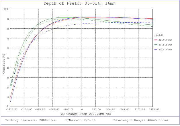
#36-514, 16mm f/5.6, HPr Series Fixed Focal Length Lens, Depth of Field Plot, 2000mm Working Distance, f5.6
