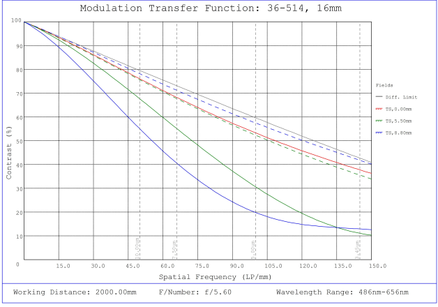
#36-514, 16mm f/5.6, HPr Series Fixed Focal Length Lens, Modulated Transfer Function (MTF) Plot, 2000mm Working Distance, f5.6
