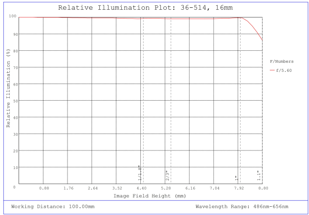
#36-514, 16mm f/5.6, HPr Series Fixed Focal Length Lens, Relative Illumination Plot
