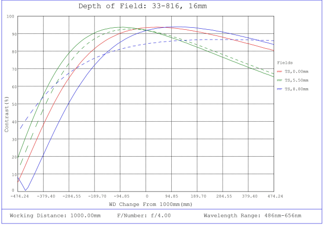
#33-816, 16mm f/4, HPI Series Fixed Focal Length Lens, Depth of Field Plot, 1000mm Working Distance, f4
