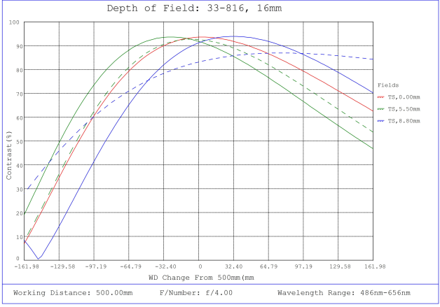
#33-816, 16mm f/4, HPI Series Fixed Focal Length Lens, Depth of Field Plot, 500mm Working Distance, f4
