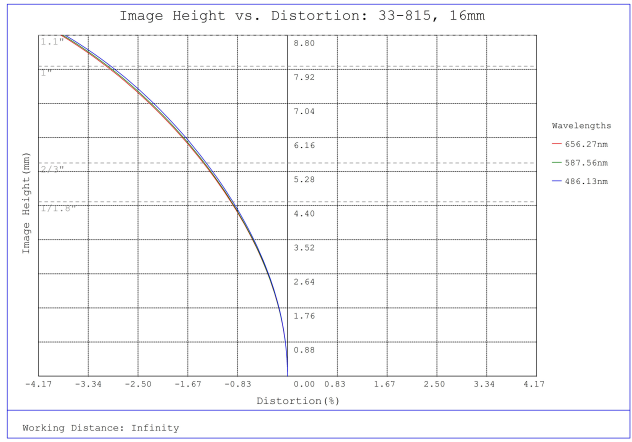
#33-815, 16mm f/2.8, HPI Series Fixed Focal Length Lens, Distortion Plot
