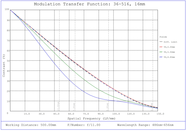
#36-516, 16mm f/11, HPr Series Fixed Focal Length Lens, Modulated Transfer Function (MTF) Plot, 500mm Working Distance, f11
