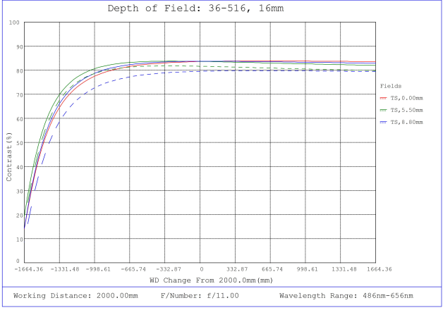
#36-516, 16mm f/11, HPr Series Fixed Focal Length Lens, Depth of Field Plot, 2000mm Working Distance, f11
