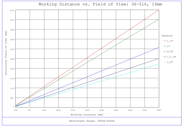
#36-516, 16mm f/11, HPr Series Fixed Focal Length Lens, Working Distance versus Field of View Plot
