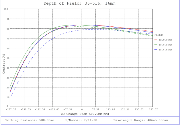
#36-516, 16mm f/11, HPr Series Fixed Focal Length Lens, Depth of Field Plot, 500mm Working Distance, f11
