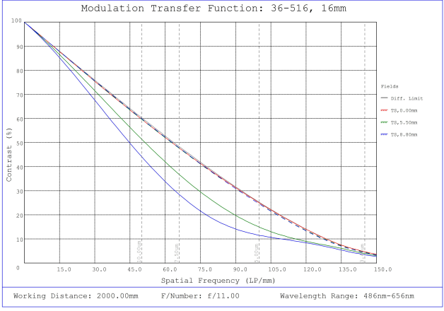
#36-516, 16mm f/11, HPr Series Fixed Focal Length Lens, Modulated Transfer Function (MTF) Plot, 2000mm Working Distance, f11
