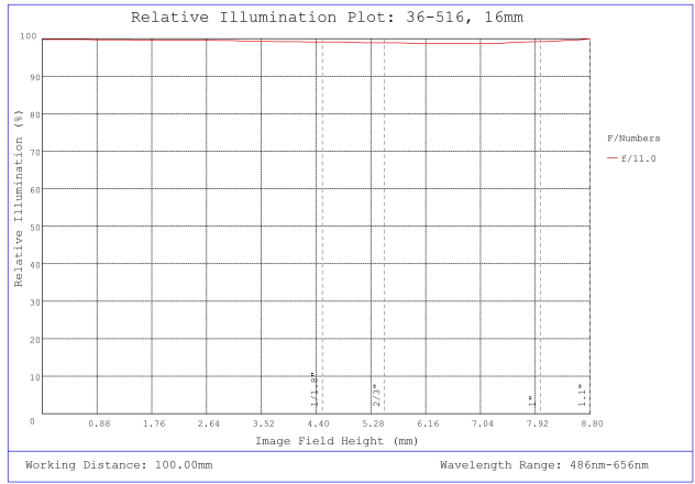
#36-516, 16mm f/11, HPr Series Fixed Focal Length Lens, Relative Illumination Plot
