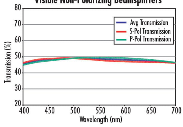
Visible Non-Polarizing Beamsplitters
