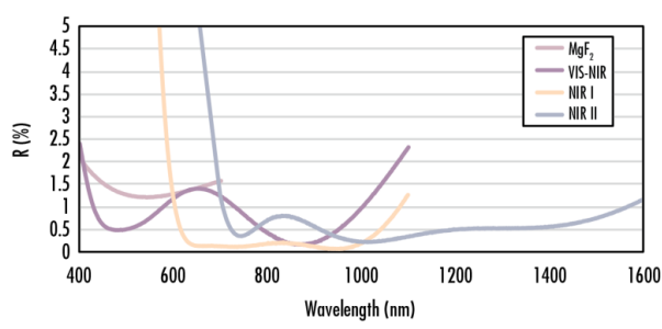
Standard Visible & NIR AR Coatings on Sapphire
