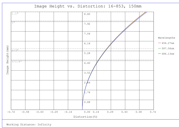
#16-853, 150mm, f/5.6 Athermal Lens, Distortion Plot
