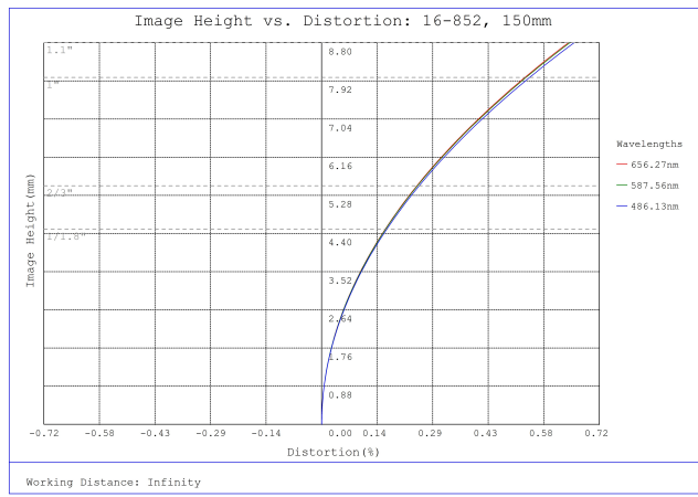
#16-852, 150mm, f/4 Athermal Lens, Distortion Plot
