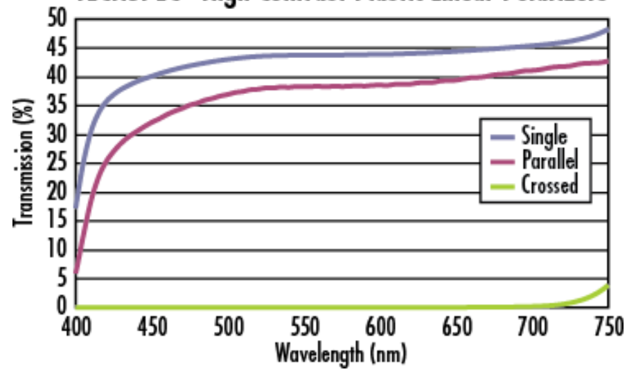
XP42 – Linear Polarizer
