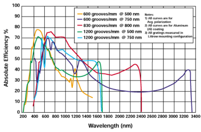
Typical Efficiency Curves for Ruled Gratings Optimized (Blaze) Wavelengths from 500-800 nm
