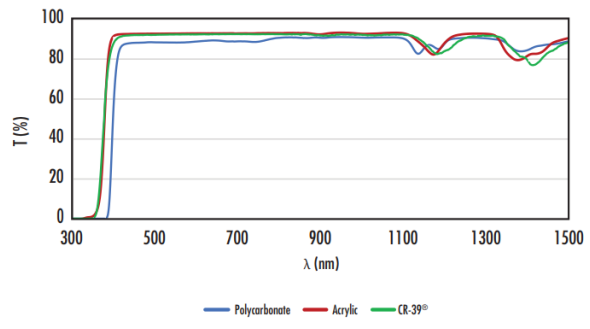
Typical Transmission of Plastic Windows
