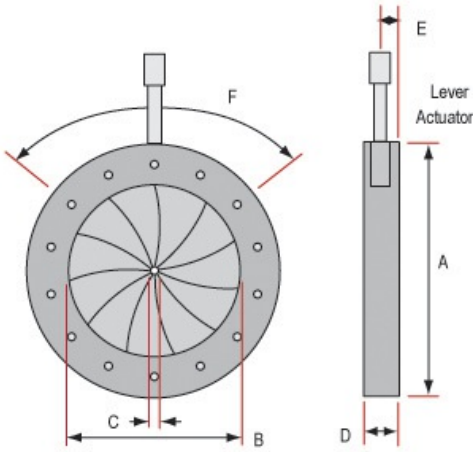
High Performance Iris Diaphragms
